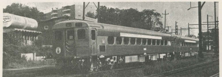
Department of Commerce high-speed test cars No. T-1 and T-2 at Jenkintown, Pennsylvania on the electrified West Trenton line of the Reading Company. After a short break-in period, the four MU cars will be returned to The Budd Company's Red Lion Plant for minor adjustments prior to the late summer commencement of the 160 mph tests on the Pennsylvania Railroad between Trenton and New Brunswick, New Jersey.
